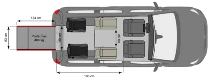
VERSION FIXE 4 PLACES
